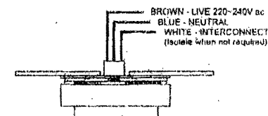
Figure 4.i - Wiring for single smoke detector
