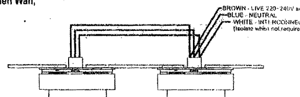
Figure 4.ii - Wiring for multiple smoke detectors (40 max)
