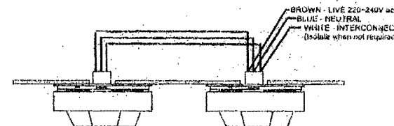
Figure 4.ii - Wiring for multiple smoke detectors (40 max)
