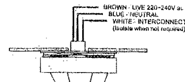
Figure 4.i - Wiring for single smoke detector
